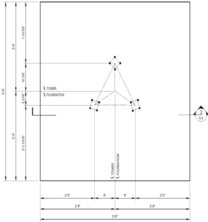
FOUNDATION PLAN 1 S-3
