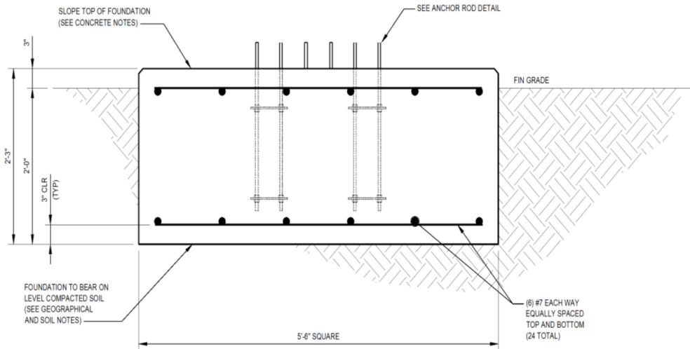
FOUNDATION ELEVATION 2 S-3
