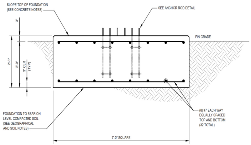
FOUNDATION ELEVATION 2 S-3
