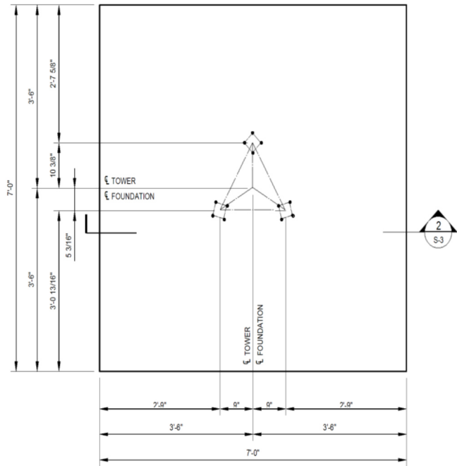
FOUNDATION PLAN 1 S-3
