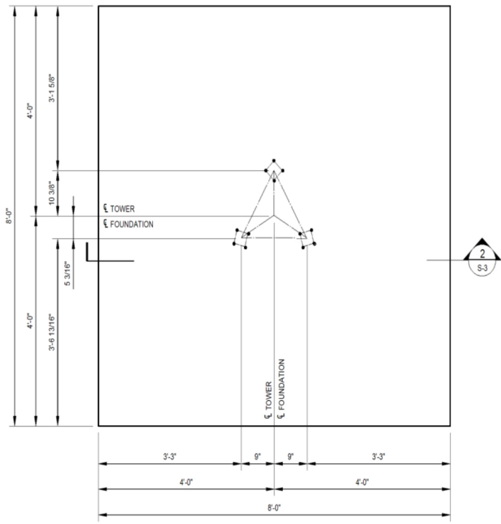
FOUNDATION PLAN 1 S-3
