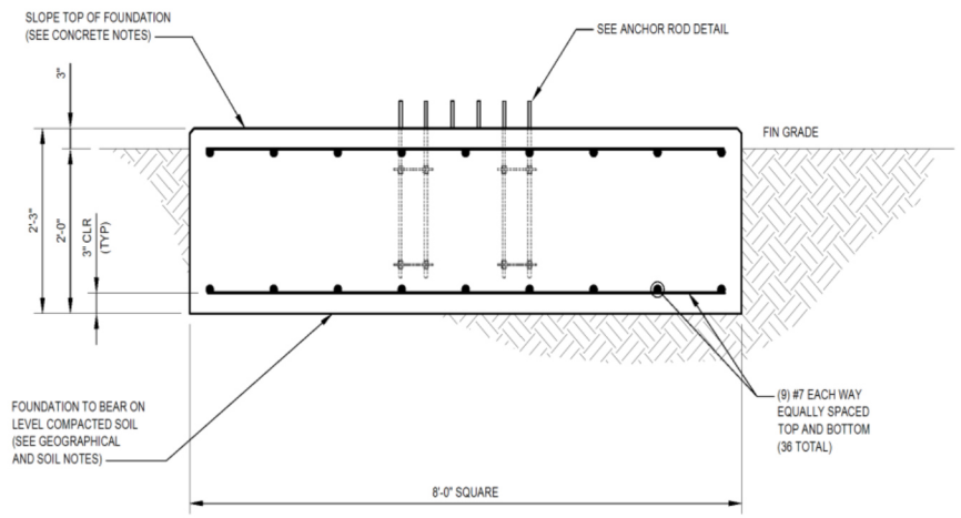
FOUNDATION ELEVATION 2 S-3
